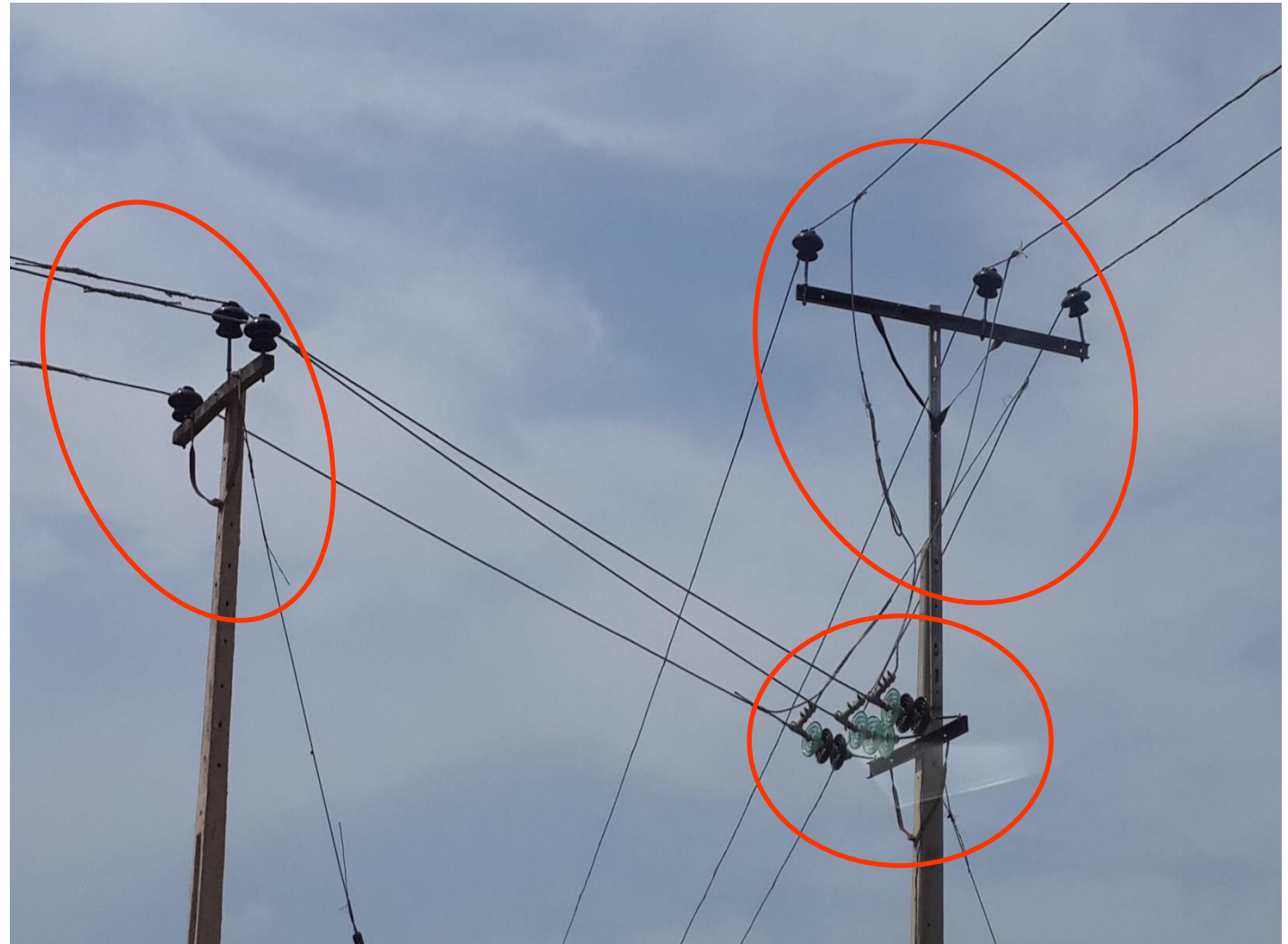
Poor terminations and dangerous Tees-off and road crossing at Kuje, FCT one year after being reported
