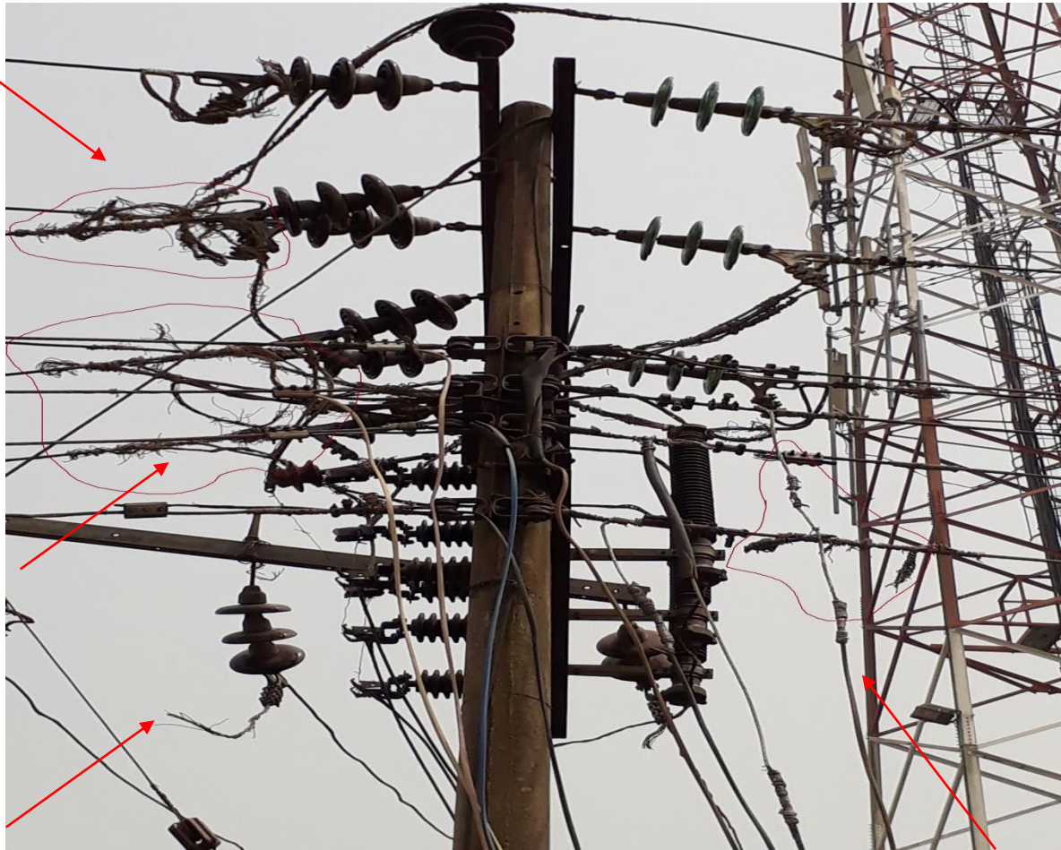
This section pole was seen carrying two outgoing 33kV feeders and two service lines. The termination joints were very badly done. The only seen neutral return conductor for the service lines was observed to be at the verge of snapping. The interwoven/cobweb of interconnections is an accident waiting to happen. Added to this is the closeness to a communication mast. [Orlu]
