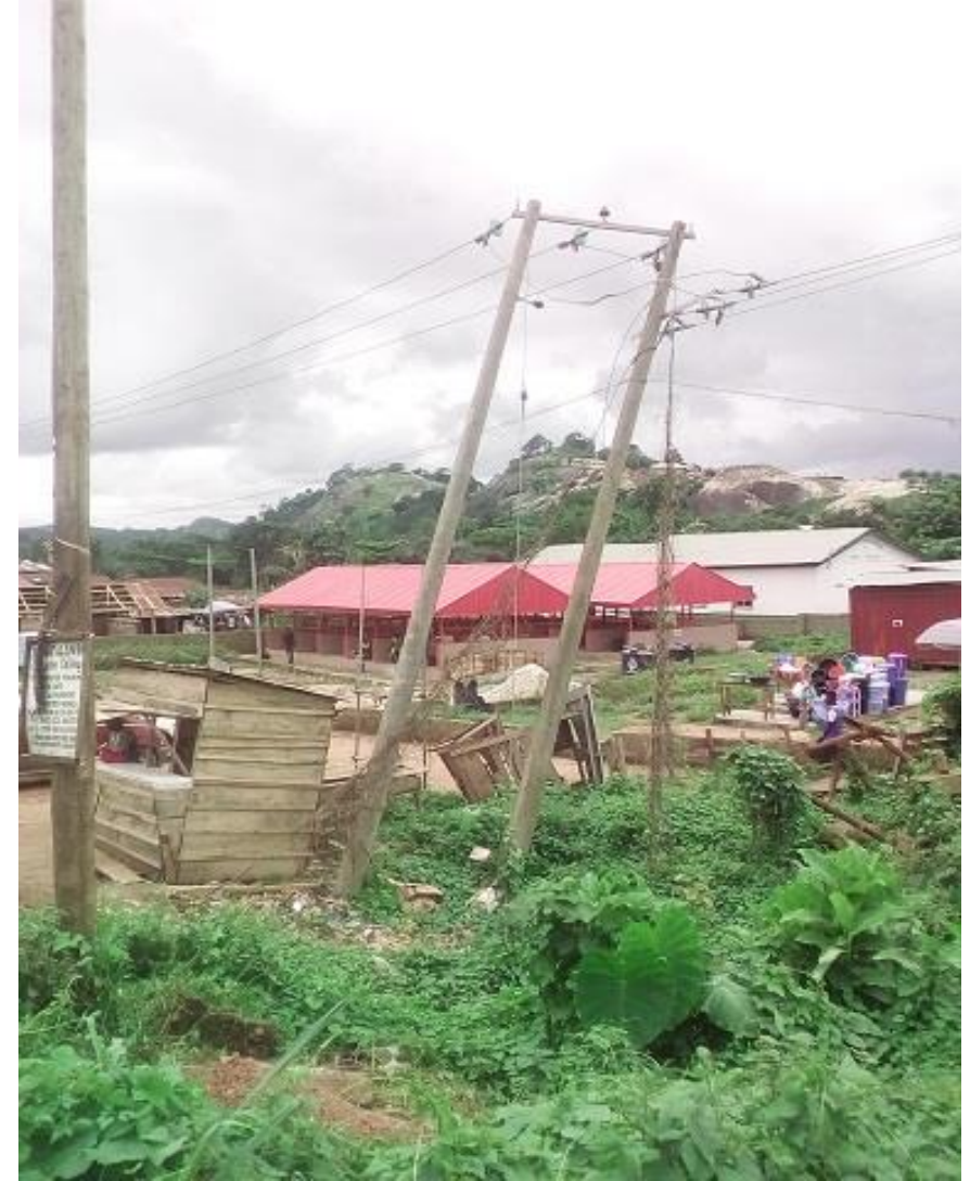
Dangerously tilted H-Pole at Adebowale Junction, Ondo Road, Akure, Ondo State.
